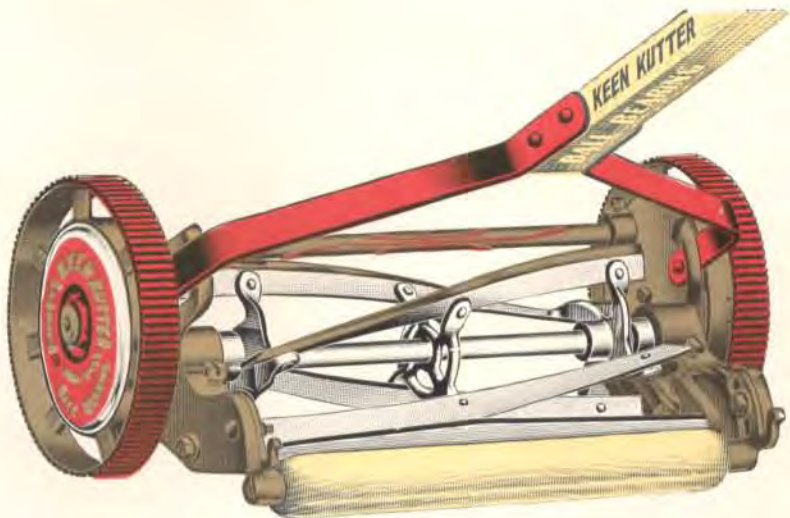
LOW WHEEL—DRIVE WHEELS 8 INCHES IN DIAMETER, 1½-INCH TREAD
