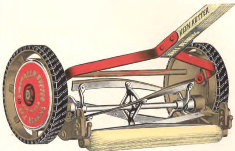
HIGH WHEEL—DRIVE WHEELS 10 INCHES IN DIAMETER, 1½-INCH TREAD
